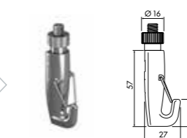
Auto Grip Lock 2.5 mm 6100.110 100 kg
